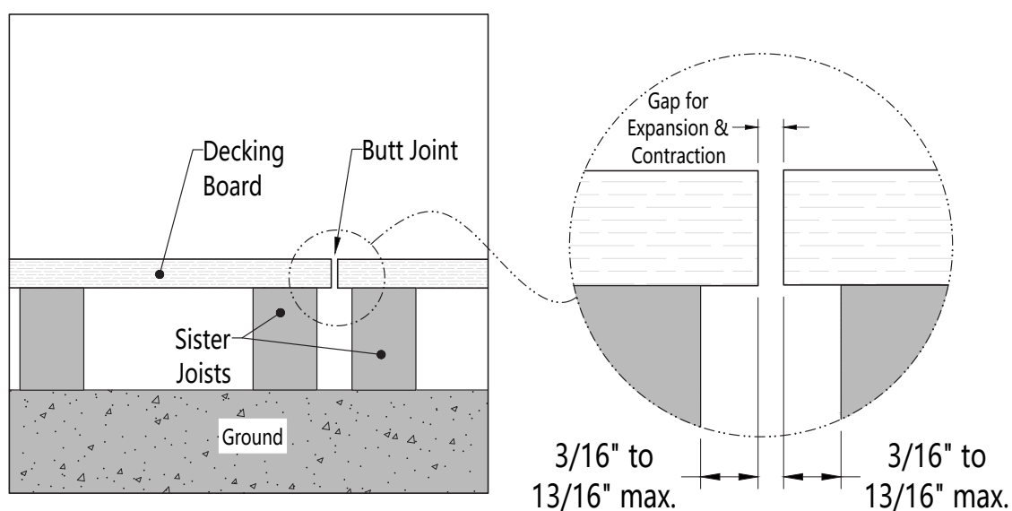
Detail 7-1
