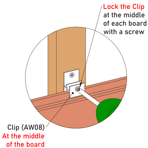
Detail 33-1
