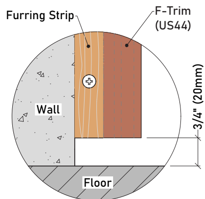
Detail 15-2
