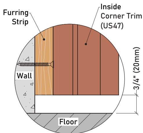
Detail 7-2
