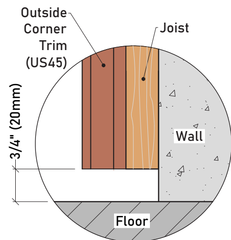
Detail 39-2
