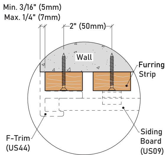
Detail 6-1
