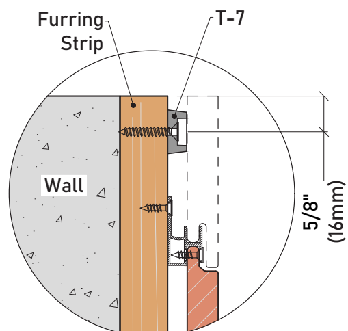
Detail 44-1
