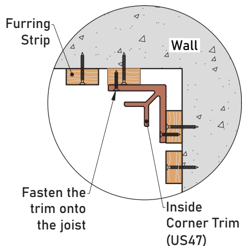
Detail 7-1
