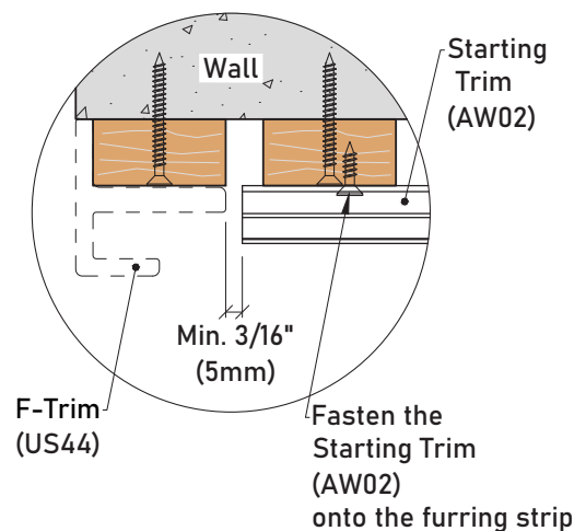
Detail 8-3
