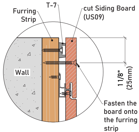
Detail 45-1
