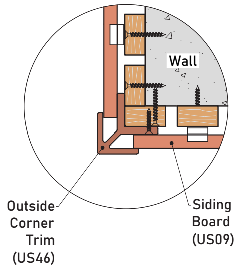
Detail 45-2
