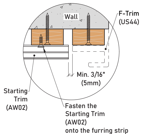
Detail 40-2
