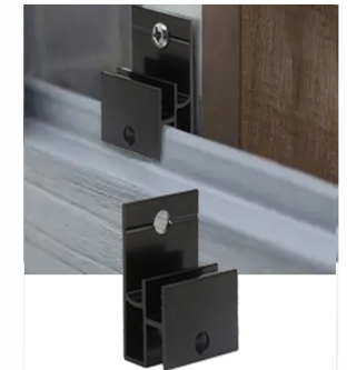
AW08 siding clips 90 per bag, 50 sqft per bag
