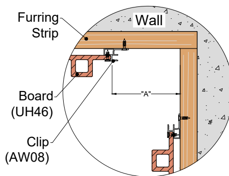
Detail 23-3
