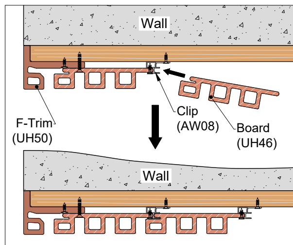
Detail 22-2
