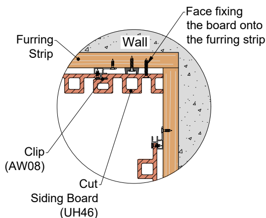
Detail 26-4
