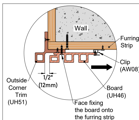
Detail 21-3
