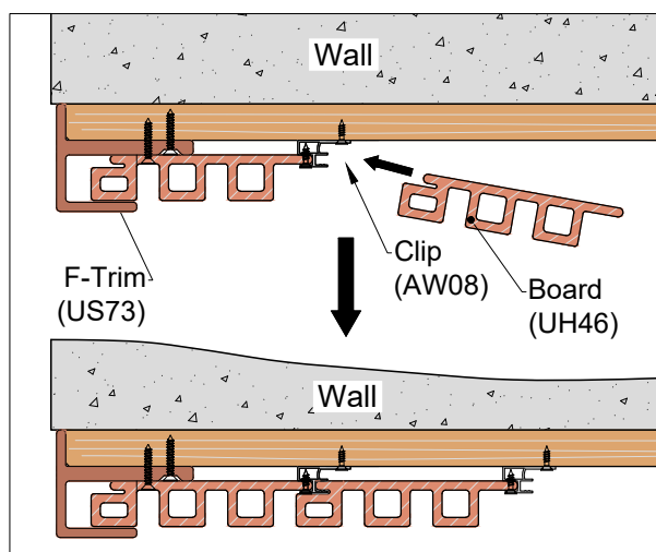
Detail 22-3
