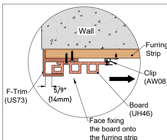
Detail 21-2
