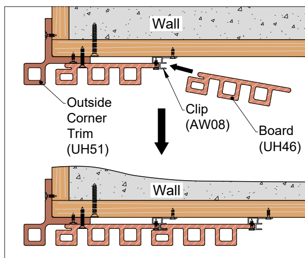
Detail 22-4
