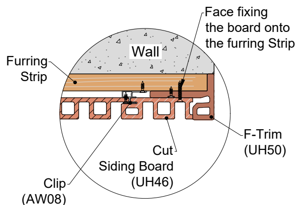
Detail 26-1
