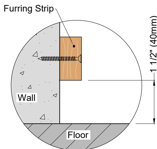
Detail 18-1
