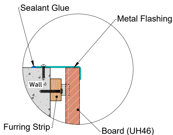
Detail 27-1
