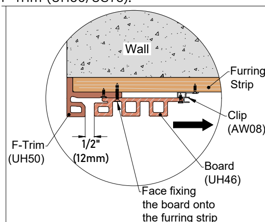
Detail 21-1
