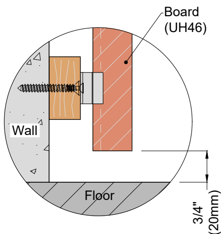
Detail 21-5
