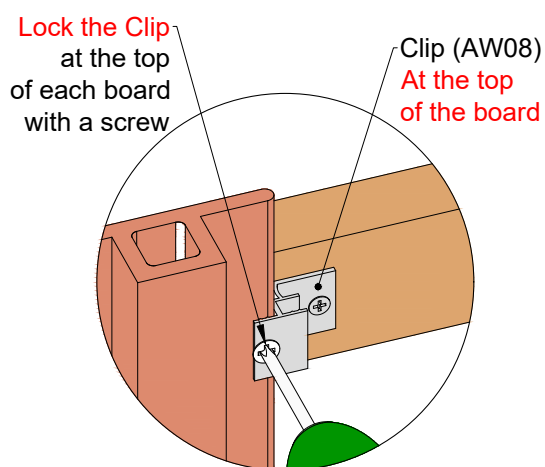
Detail 22-1
