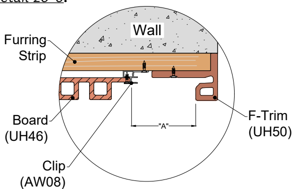
Detail 23-1
