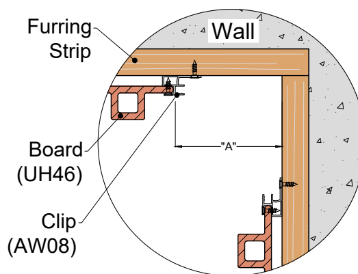
Detail 23-4
