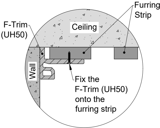
Detail 3-1
