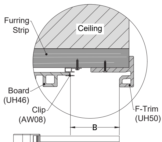
Detail 10-1
