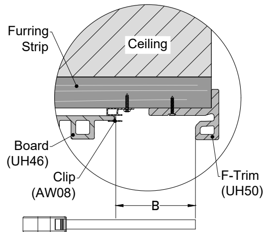
Detail 10-1
