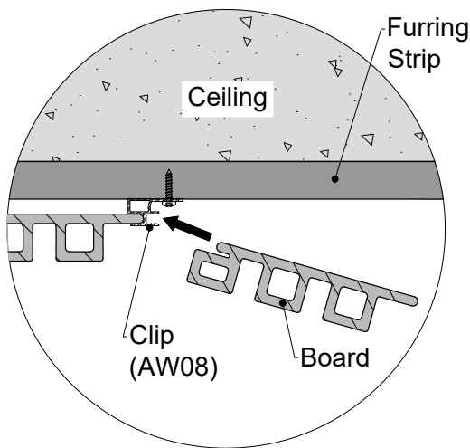
Detail 9-1
