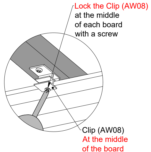
Detail 8-1
