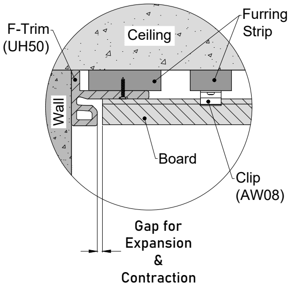
Detail 7-2
