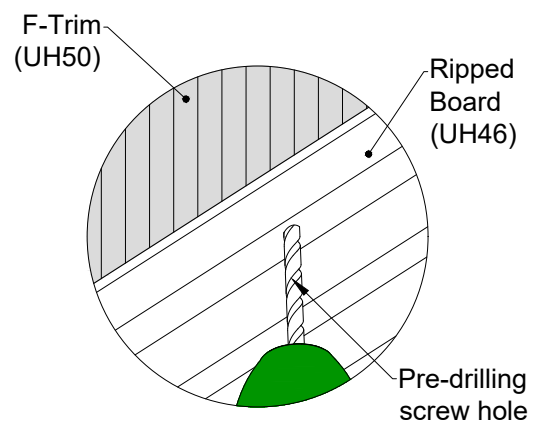
Detail 12-1
