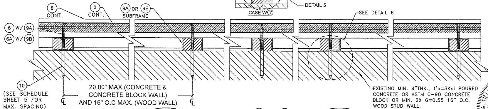
SECTION C-C
