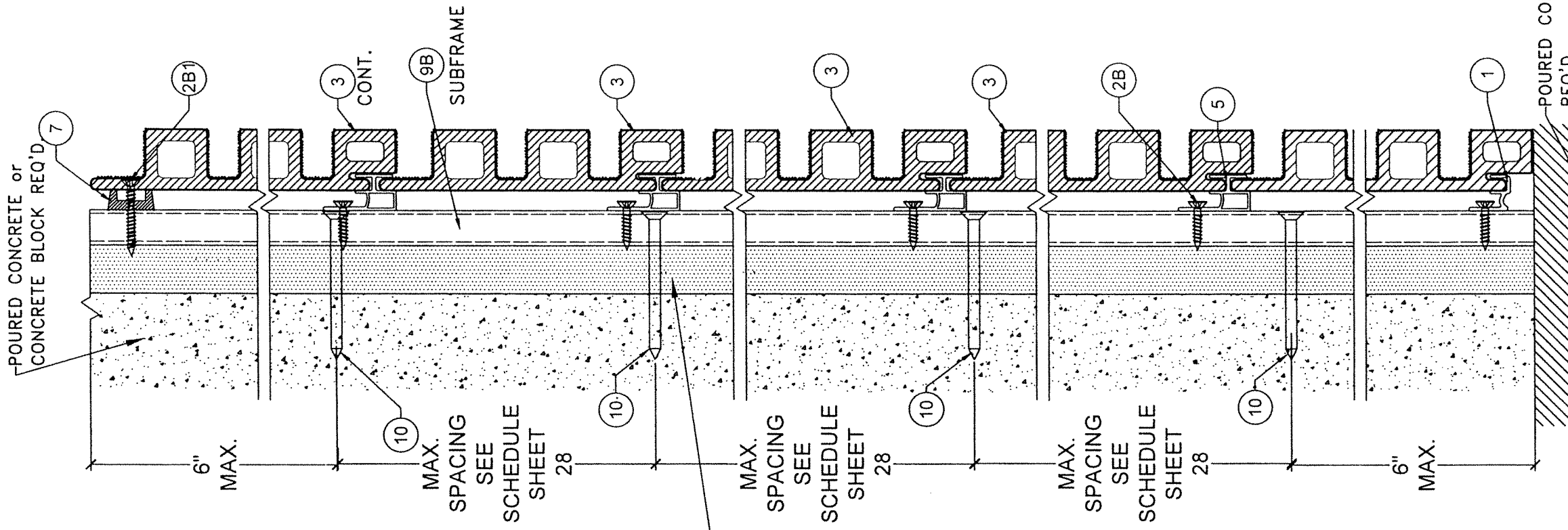
DETAIL 7
