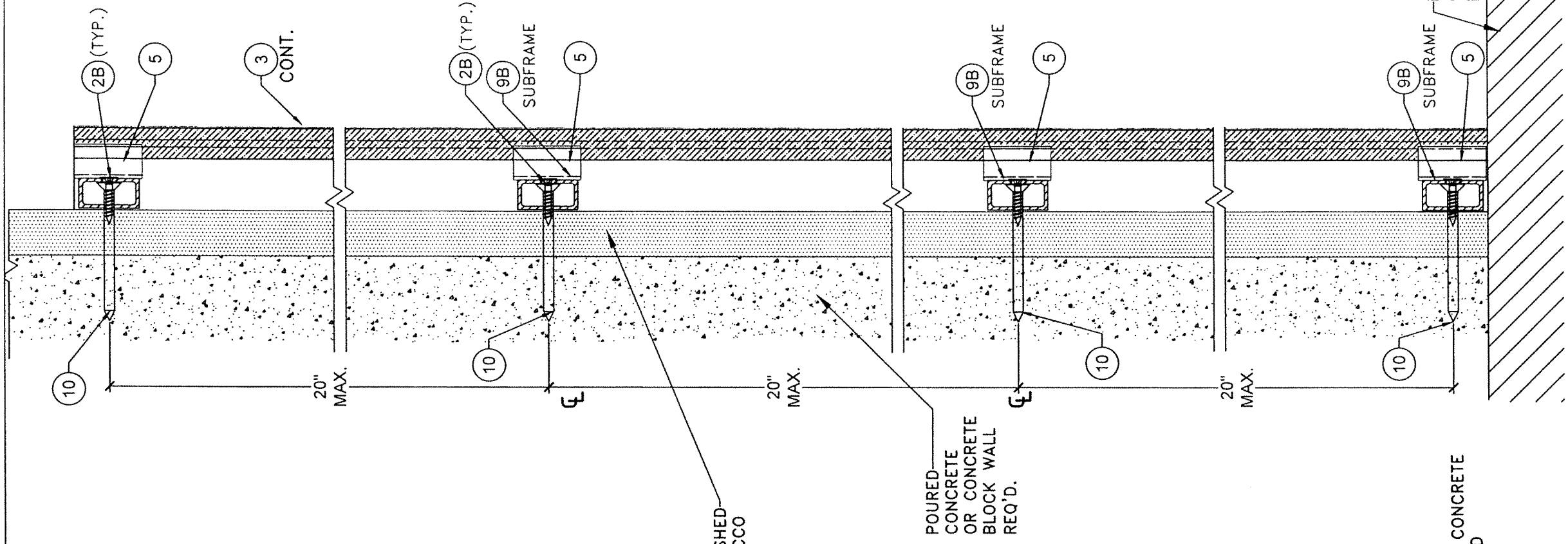
DETAIL 7
